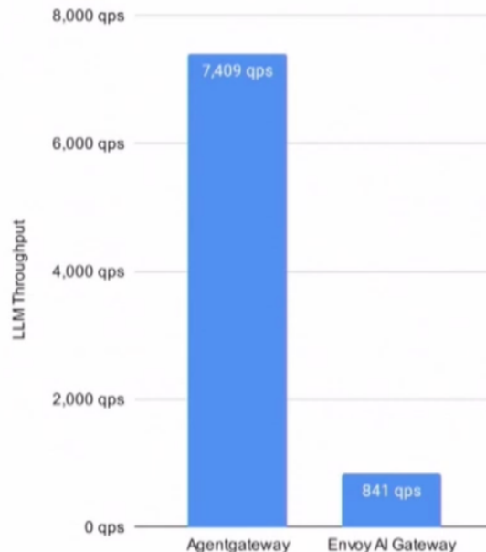
LLM Throughput
